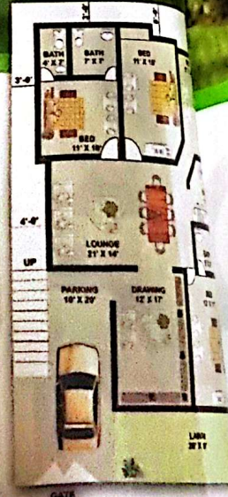
240 Sq.Yds. SINGLE STOREY GROUND FLOOR PLAN
