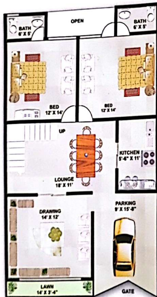
120 Sq.Yds. ONE UNIT GROUND FLOOR PLAN
